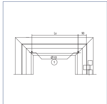
Safety sensor drill hole distances opposite hinge side
