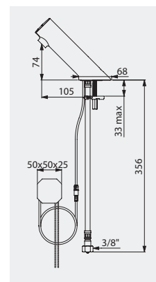
TEMPOMATIC 5 tap, mains supply Ref. DELABIE: 449100
