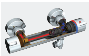
H9768TP cut-away: low water volume, thermal insulation and no non-return valves Ref. DELABIE: Coupe3D_H9768TP + 880
